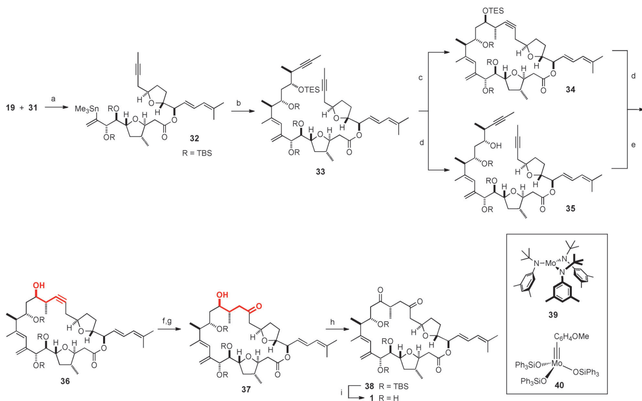
Scheme 6. a) 2,4,6-Trichlorobenzoyl chloride, \text{Et}_3\text{N} , DMAP, toluene, 80%; b) 14 , [\text{Pd}(\text{PPh}_3)_4] (30 mol %), \text{Ph}_2\text{PO}_2\text{NBU}_4 , CuTC, DMF, 56%; c) 39 (30 mol %), toluene, \text{CH}_2\text{Cl}_2 , 60 °C, 73%; d) PPTS (30 mol %), MeOH, \text{CH}_2\text{Cl}_2 , 0 °C, 87% ( 36 ), 95% ( 35 ); e) 40 (20 mol %), toluene, 100 °C, 70%; f) [\{(\text{C}_2\text{H}_4)_4\text{PtCl}_2\}_2] (0.2 mol %), \text{Et}_2\text{O} , 97%; g) PPTS, benzene, 98%; h) TPAP, \text{CH}_2\text{Cl}_2 , 70%; i) HF-NEt 3 , \text{Et}_3\text{N} , MeCN, 40 °C, 60%; CuTC = copper thiophene-2-carboxylate; DMAP = 4-dimethylaminopyridine; TPAP = tetra- n -propylammonium perruthenate
